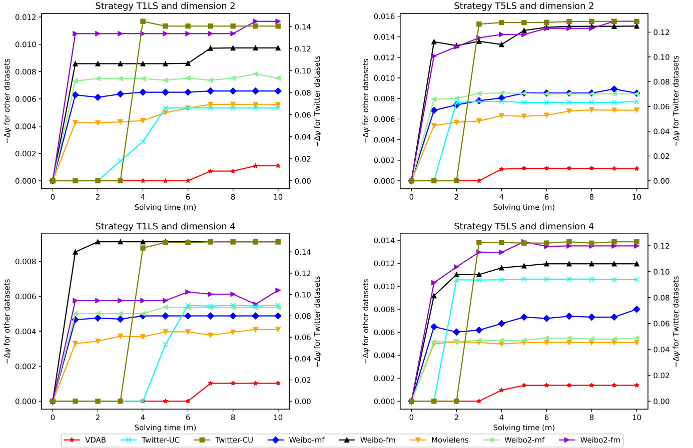
Fig. 4: Amount of imbalance reduction -\Delta\psi against solving time for mapping variables ratio r with the highest imbalance reduction r for dimensions 2 and 4 and candidate link strategy T1LS and T5LS. Note a different scale is used for the Twitter datasets, hence there is a double y-axis.
