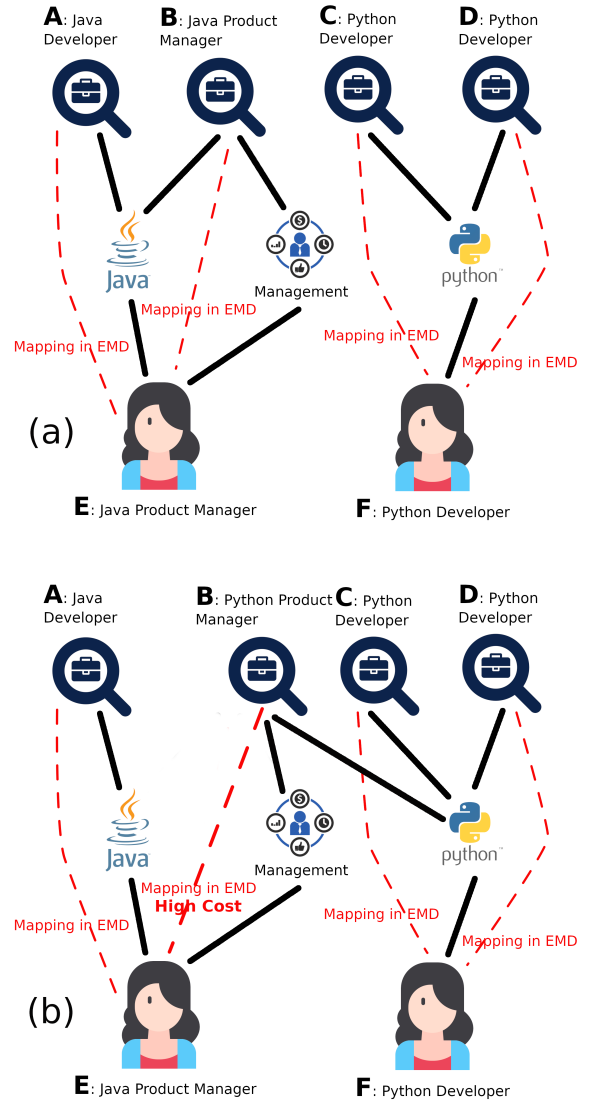
Fig. 1: A sample job market. A, B, C, and D are job positions and E and F are job seekers. E is a Java product manager and F is a Python developer. Solid lines are the links in the original graph. Dashed lines give the mapping that minimizes the EMD. (a) A and B are Java related job positions and C and D are Python related job positions. (b) A is a Java related job position and B, C, and D are Python related job positions. Note that in both cases B is about product management, whereas A, C, and D are developer positions. Since there are four job positions available and two people are seeking jobs in the example, the ideal case is (a) where there are two job positions with low mapping costs for each of the job seekers. On the other hand, in (b) there is an imbalance in the job market where one job seeker (F) can be mapped to two job positions with low costs (C and D), and the other job seeker (E) can be mapped to only one job position (A) with a low cost, while for one job (B) there is no ideal candidate available. Giving all nodes per type equal weight, the EMD maps each job seeker to a fixed number of job positions. The EMD for (b) is high, due to the high cost of mapping the Java product manager (E) to one of the Python related job positions (e.g., B). Hence, the EMD corresponds to the degree of imbalance in the job market.
