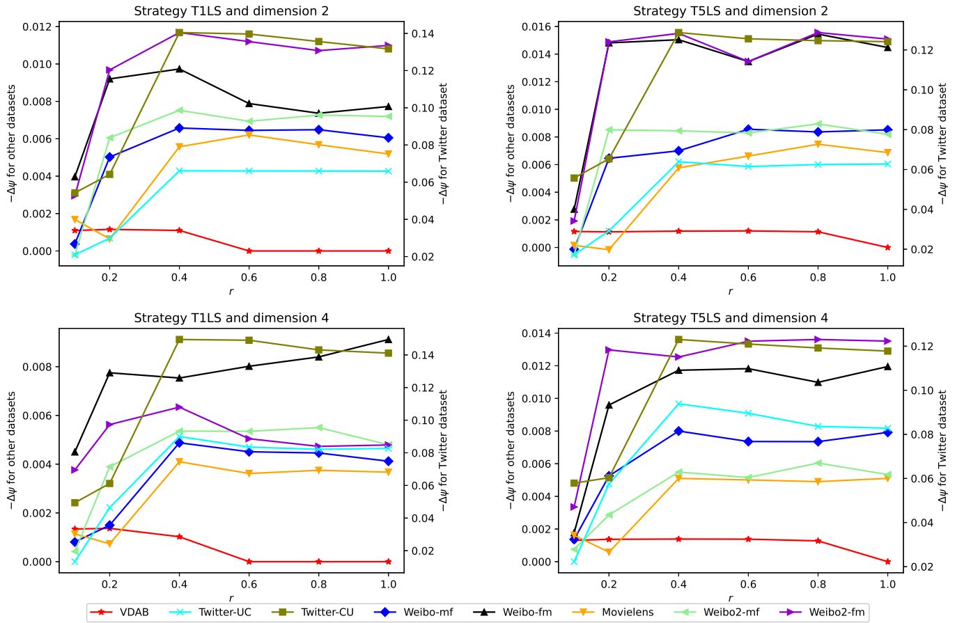
Fig. 3: Amount of imbalance reduction -\Delta\psi against matching variables ratio r for dimensions 2 and 4 and candidate link strategy T1LS and T5LS. Note a different scale is used for the Twitter datasets, hence there is a double y-axis.
