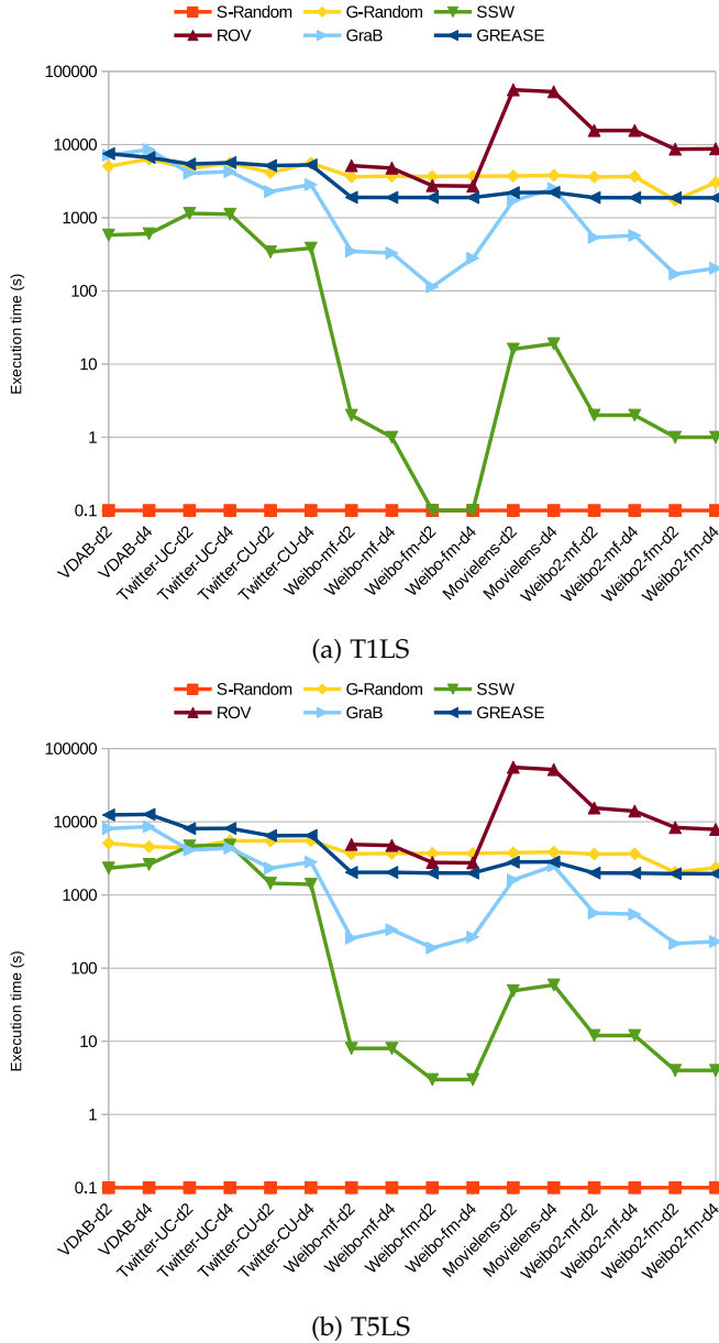
Fig. 2: Execution time (log-scale) of methods for experiment 5.4.1 on each evaluated network for candidate set strategies T1LS and T5LS. Since the y-axis is in log-scale, 0.1 is used to represent all values between zero and 0.1.
