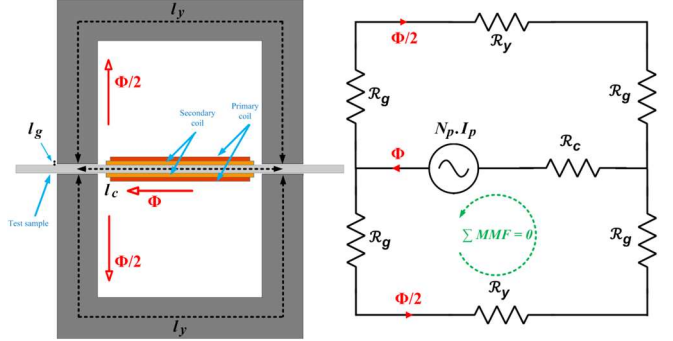
Fig. 7. Magnetic equivalent circuit model of the used single sheet tester.
