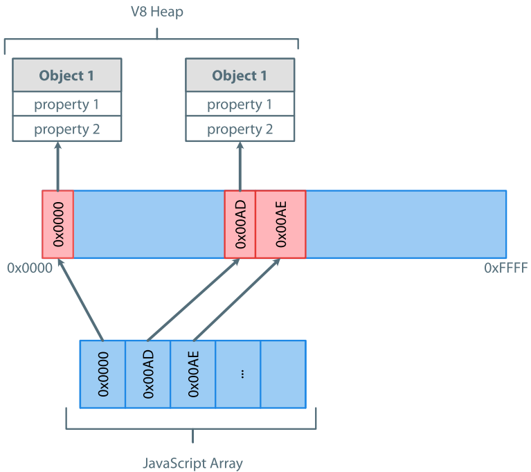
Figure 7.13: Only references to JavaScript objects are stored in an array, not the data that makes up the objects themselves. This means that if 2 arrays point to the same objects, the objects themselves are only kept once in memory!
