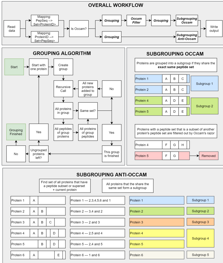
Figure 7.6: Algorithmic workflow of Pout2Prot. The general workflow is visually represented in Overall Workflow (top). The (sub)grouping building blocks of this workflow are visually represented as well: the general grouping algorithm (middle, left), the subgrouping algorithm of Occam's razor (middle, right), and the subgrouping algorithm of anti-Occam's razor (bottom).
