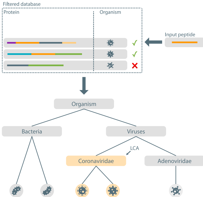
Figure 3.2: An example of how the lowest common ancestor (LCA) for a set of identified taxa is computed in Unipept Desktop, using a filtered protein reference database. The reference database is restricted to viral proteins only and a much more specific LCA will be found (mapping onto the Coronaviridae family). This example illustrates the importance of targeted protein reference databases when analyzing metaproteomics samples.
