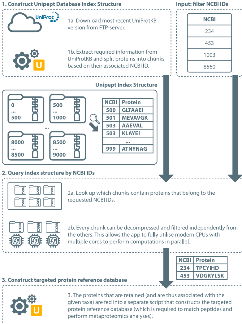
Figure 3.5: To efficiently filter the UniProtKB database, Unipect builds a custom index structure that can be easily filtered by taxon ID. This index structure only needs to be built the first time and will be reused for all subsequent database builds. The NCBI taxon IDs, optionally provided by a user, are used to select which index chunks need to be queried. Each of these chunks is a compressed file containing protein information, which can then be processed in parallel by multiple CPU-cores.
