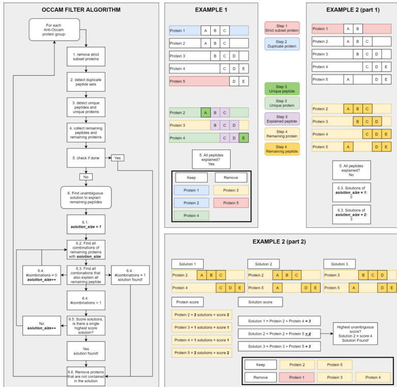
Figure 7.7: The Occam Filter algorithm visually represented (left), including two examples (right).
