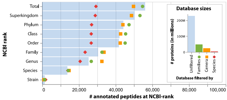
Figure 3.6: Four analyses have been performed on the same metaproteomic sample, but with a different underlying protein reference database. In the main visualization (left), we compare the number of peptides with a taxon match at a specific rank (or lower) in the NCBI taxonomy. In most cases the analyses performed by using a reference database constructed from families or genera performs as well as or better than the full UniProtKB database. However, these databases contain only a fraction of the proteins (right) and therefore require much less computational resources. At the species level, all protein reference databases behave almost identically. At higher ranks, we can see that the reference database constructed from a set of species is probably too restricted.
