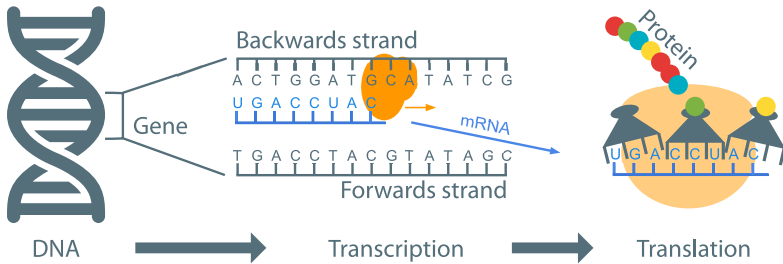
Figure 1.3: Schematic depiction of how information recorded in a gene is converted (or synthesized) into a protein. The DNA in a gene is first converted to mRNA (transcription). The mRNA will then be read in groups of 3 nucleotides at a time and matched with amino acids. The final sequence of amino acids constructed this way corresponds with a protein.
