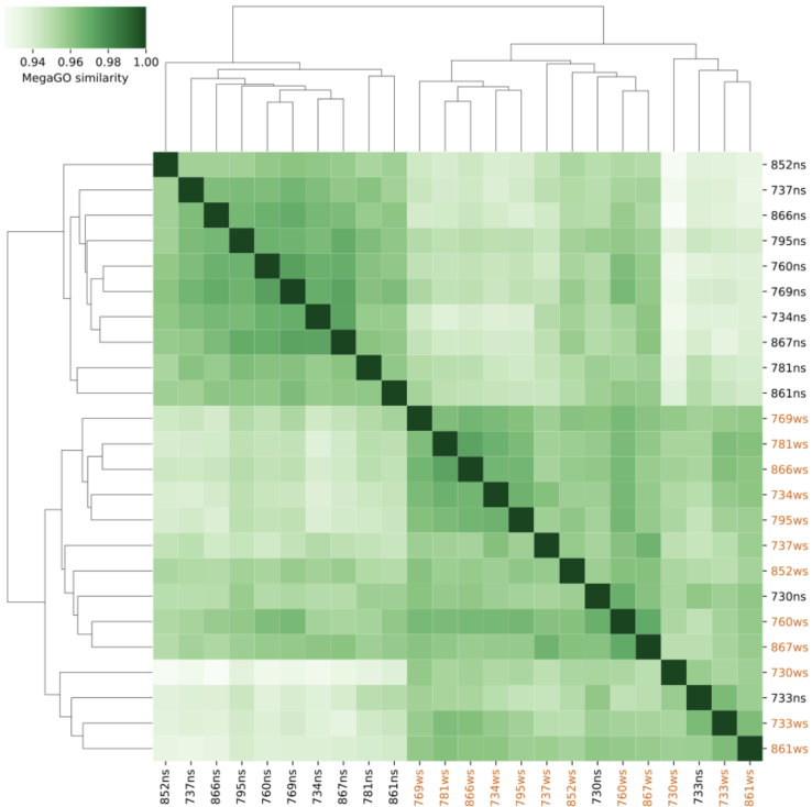
Figure 6.4: Hierarchically clustered heatmap comparing MegaGO similarities for the GO domain “biological process” for each of the samples from (Easterly et al. , 2019). Samples that are treated with sucrose pulsing are labeled as “ws” and are displayed in orange.
