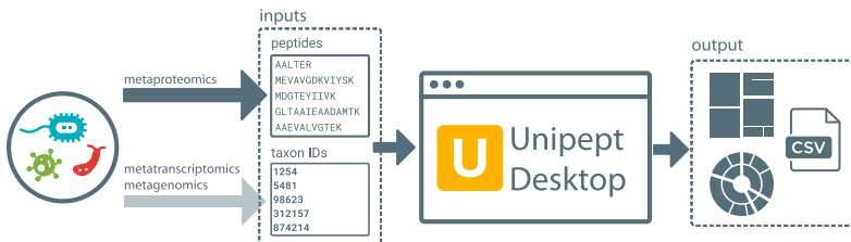
Figure 3.3: Unipept Desktop application analysis pipeline. The Unipept Desktop application requires a list of peptides to perform a taxonomic and functional analysis on and optionally accepts a list of NCBI taxonomy IDs that are used to restrict which proteins are taken into account during this metaproteomics analysis. These taxonomy IDs are typically extracted from a prior metagenomics or metatranscriptomics experiment.
