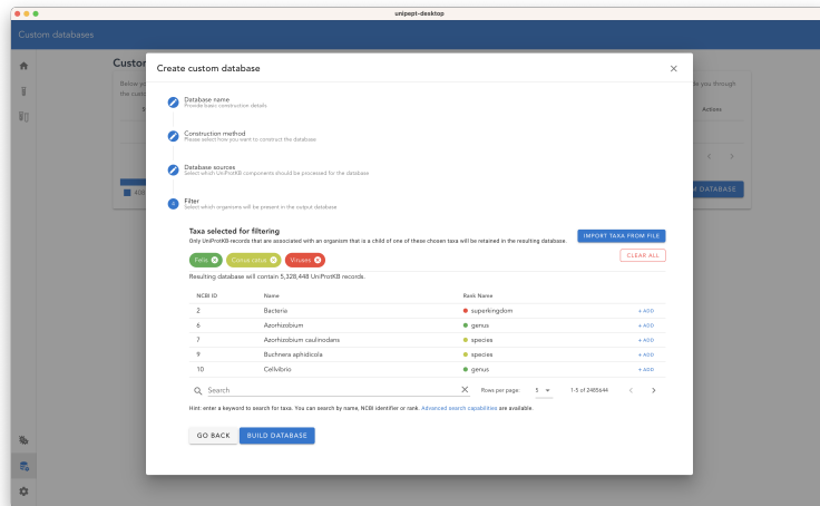
Figure 3.4: Database creation wizard in Unipept Desktop 2.0. This wizard guides the user through the process of building a targeted protein reference database. Researchers can select proteins in two different ways: by providing a set of taxon identifiers, or by providing a list of UniProtKB reference proteome IDs.
