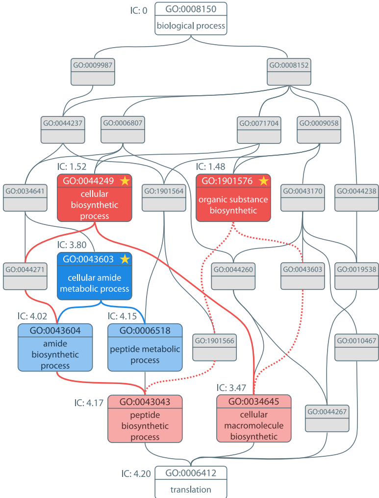
Figure 6.2: Excerpt of the biological process domain of the Gene Ontology showing all parent terms up to the root for “translation” (GO:0006412). IC, information content; *, most informative common ancestor.
