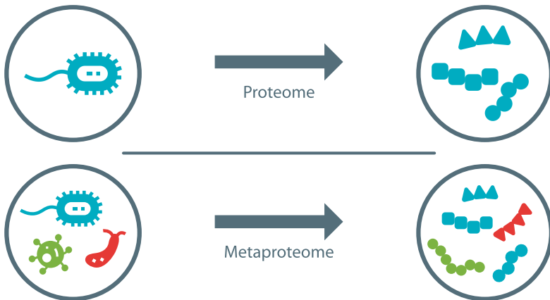
Figure 1.4: A schematic overview of the proteome and the metaproteome. The proteome is defined as the proteins that can be expressed by a single organism. The metaproteome, on the other hand, is then defined as the set of proteins that can be defined by a collection of organisms.
