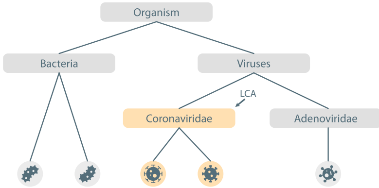
Figure 1.11: If the organisms in orange are selected, the lowest common ancestor of these organisms in the NCBI taxonomy will be Coronaviridae , because this is the most specific node that is a parent of both organisms.
