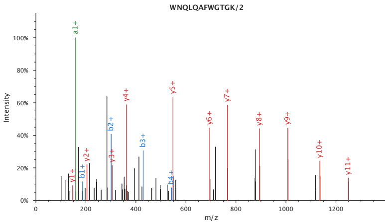
Figure 1.7: Example of a mass spectrum for the peptide WNQLQAFWGTGK/2, taken from (Bittremieux, 2020). The different peaks in the spectrum correspond with the observed “mass-to-charge” ratio of the different particles of the input sample.
