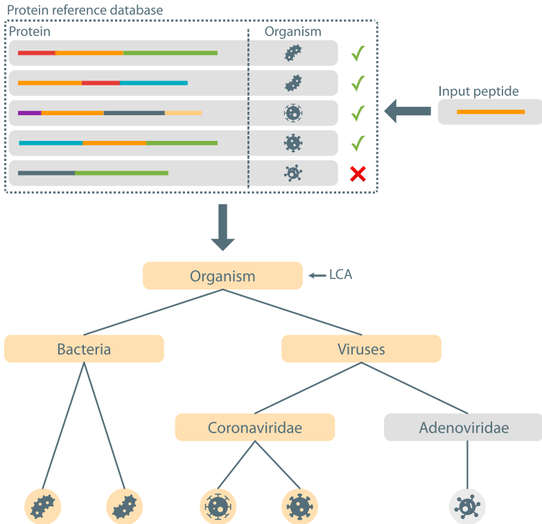
Figure 3.1: An example of how the lowest common ancestor (LCA) for a set of identified taxa is computed in Unipept Desktop, using an unfiltered protein reference database. A single input peptide is matched against proteins in a reference database. The taxa associated with all matched proteins are then summarized as the LCA, which is the most specific node in the taxonomy tree that is a parent of all matched taxa. An unfiltered protein reference database is used in the matching process. Since more proteins from a more diverse range of species are matched, the LCA ends up at the root of the taxonomy tree, providing little to no information. b) The reference database is restricted to viral proteins only and a much more specific LCA will be found (mapping onto the Coronaviridae family).
