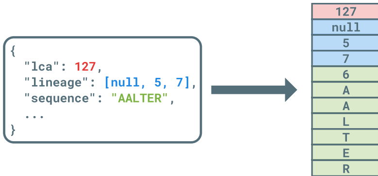
Figure 7.15: Example of how a complex object (in the case of Unipept) can be encoded as a simple stream of bytes that directly fits into an ArrayBuffer. We know that the lowest common ancestor is always an unsigned integer, so we can store it in the first 4 bytes of a block of memory. The lineage in this example is a numeric array that always contains 3 unsigned integers, thus the next three places in the ArrayBuffer are reserved for this array. By continuing this strategy, each of the properties can directly be encoded in the memory block and can be recovered very efficiently.
