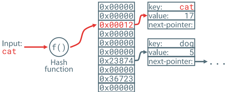
Figure 7.14: Looking up a value in the HashMap consists of several steps. First the key is hashed, then the position of this hash in the index table is computed. At last, the pointer at this computed position in the index table can be used to retrieve the value associated with the key.
