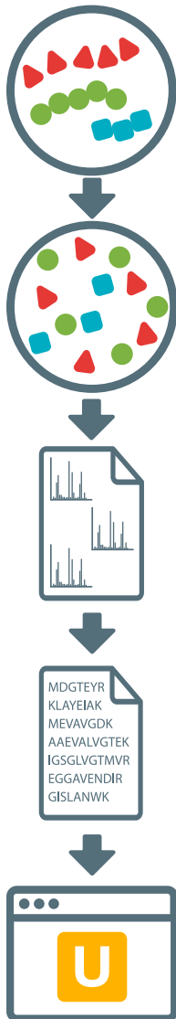
Figure 1.5: Overview of the different steps in a typical shotgun metaproteomics analysis pipeline. Each step comes with its own set of challenges that need to be overcome for which dedicated tools have been developed.
