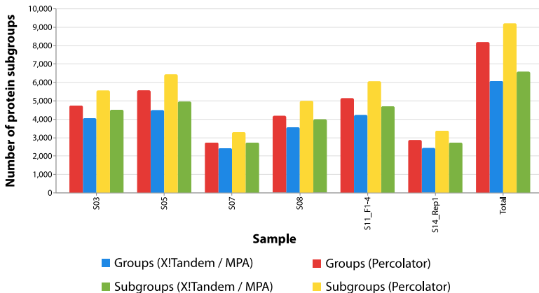
Figure 7.5: Number of protein (sub)groups compared between X!Tandem and Percolator for the anti-Occam's razor strategy, and number of protein (sub)groups using Percolator for the Occam's razor strategy. S03, S05, S07, S08, S11_F1-4, and S14_Rep1 refer to the six SIHUMIx samples.
