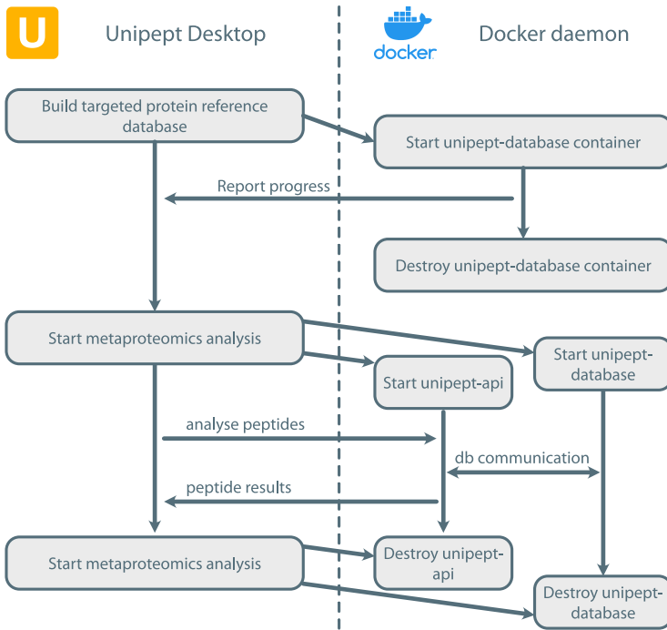
Figure 3.7: This figure is a schematic representation of the communication that takes place between the Unipept Desktop app and Docker when a user decides to analyse a metaproteomics dataset using a targeted protein reference database.
