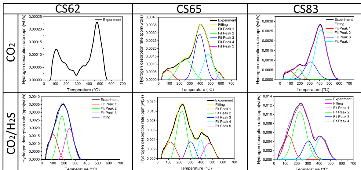
Fig. 4. TDS spectra obtained at a heating rate of 0.5 K/s for the studied materials exposed to 0.2 bar \text{CO}_2 and 0.2 bar \text{CO}_2 /1 mbar \text{H}_2\text{S} environments for 21 days at room temperature. The deconvoluted curves is associated with the H desorption from particular microstructural features. (For interpretation of the references to color in this figure legend, the reader is referred to the web version of this article.)
