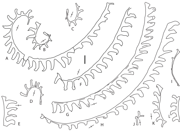
Fig. 11. Selected specimens of Demirastrites and Demirastrites? from the uppermost Rhuddanian – lower Aeronian in the Rheidol Gorge section. A–G, Demirastrites triangulatus (Harkness, 1851). A, specimen collected by Sudbury (1958), identified as Monograptus triangulatus separatus , flattened to partial relief, SM A24849, Sudbury's Horizon S (approx. 10.25–10.45 m). B, partial relief, Zx13970, 10.17–10.22 m. C, partial relief, Zx14056, 11.67–11.77 m. D, partial relief, some brittle deformation mesially, Zx14039, 10.52–10.57 m. E, partial relief, Zx13976, 10.17–10.22 m. F, partial relief, Zx14071, 11.67–11.77 m. H, I, Demirastrites? walkerae (Rickards, Hutt & Berry, 1977), all partial relief, Zx14105a, b, 12.47–12.57 m. J–L, Demirastrites? brevis (Sudbury, 1958). J, partial relief, Zx14004a, 9.82–9.87 m. K, partial relief, Zx14004b, 9.82–9.87 m. L, partial relief, Zx13983, 9.67 m. Elongate cross symbols indicate direction of tectonic lineation (bedding-cleavage intersection and/or mineral lineation) on bedding surfaces, shown for those samples where it was clearly evident. Scale bar represents 1 mm.
