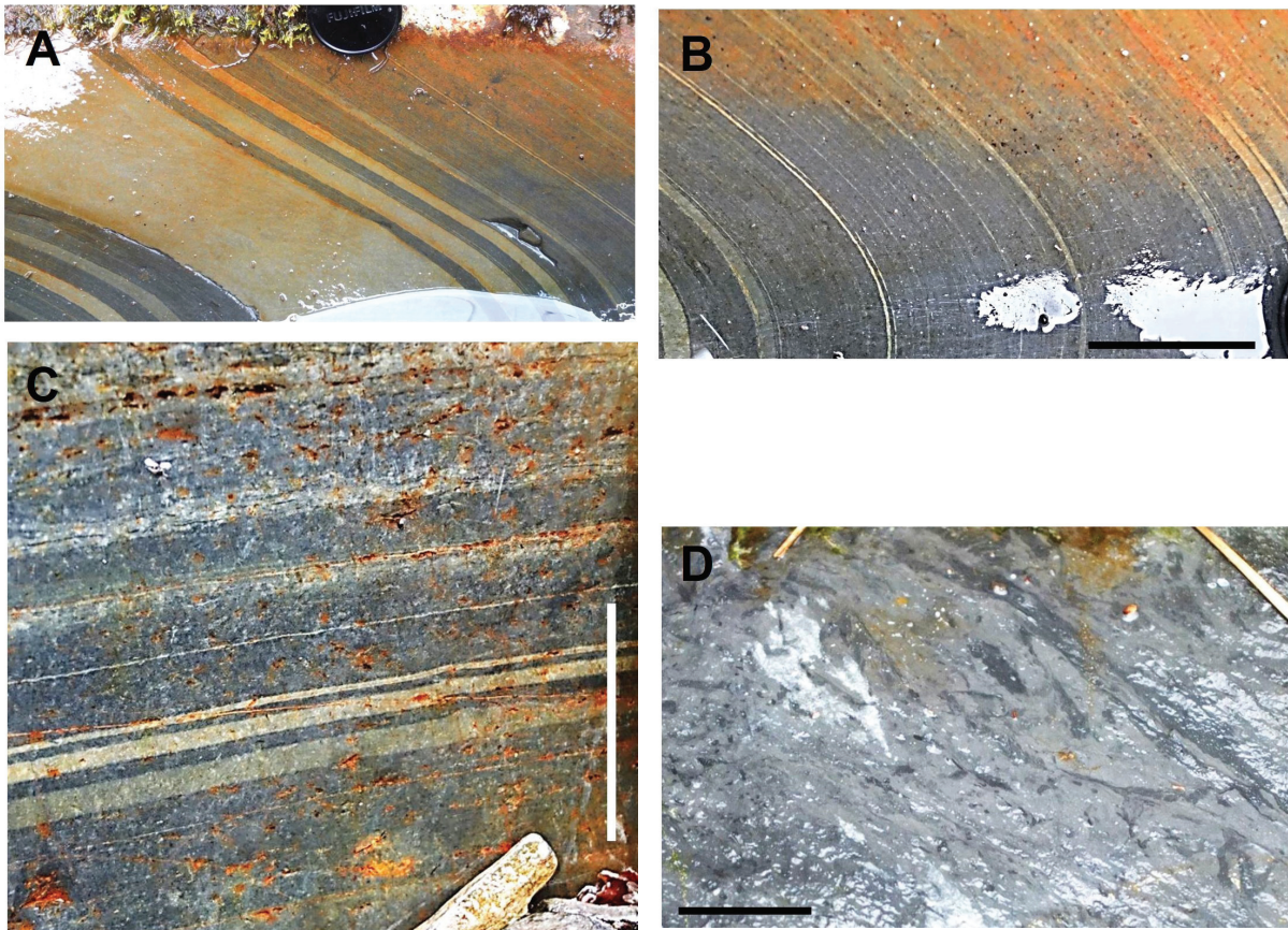
Fig. 7. Impacts of differing levels of oxicity during deposition and early diagenesis; location references refer to Figure 4 and RO values to Table 2 (see also Fig. 6). A, delicately laminated, anoxic hemipelagic mudstones (dark grey-black) with fine-grained sandstone and siltstone turbidite beds and laminae (pale grey/brown) (RO = 0), c 1.32 m, lens cap is 5 cm in diameter (note thickest turbidite bed is sandy flag G of Jones (1909). B, enhanced close-up of hemipelagic lamination in A (note well preserved varve-like alternation of dark, organic-rich and lighter silt-rich laminae), scale bar is 5 cm. C, upwards transition from dark grey, diffusely laminated hemipelagic mudstones with paler turbidite beds and laminae and sparse burrows (RO = 1) into increasingly burrow-mottled equivalents (RO = 2 to 3), c 8.9 m, scale bar is 3 cm (note more diffuse nature of the lithological contacts and more poorly preserved hemipelagic lamination in the lower facies compared with A and B and increasing levels of disruption and loss of definition upwards; D, Strongly burrow-mottled mudstone (RO = 3) at c 8.25 m, scale bar is 20 mm (note range of burrow sizes including large diameter varieties and presence of branching burrow systems).
