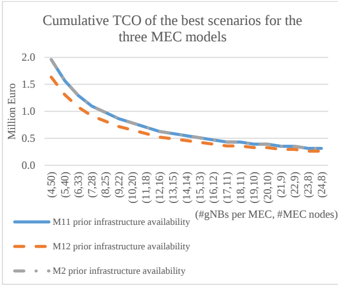
Fig. 5. The cumulative TCO as a function of the number of MEC nodes for best scenarios of the three MEC models.
