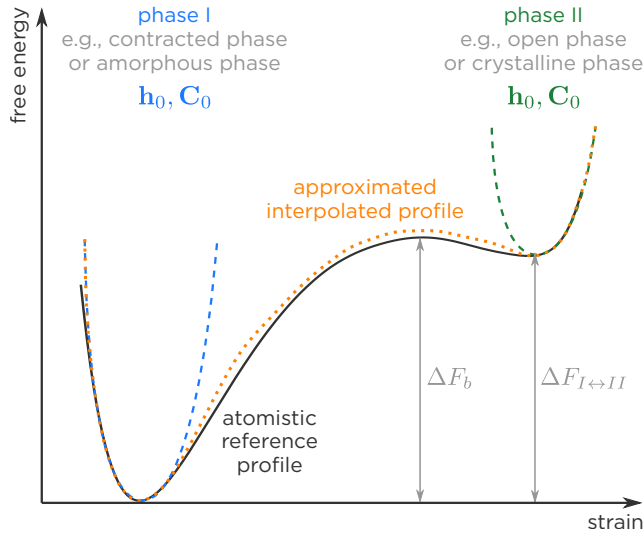
Fig. 4 Visual representation of the procedure to extend the micromechanical model to systems with multiple metastable phases. The two dashed parabola indicate the harmonic responses of the two phases, I and II, separately, while the orange dotted line is the interpolation obtained according to the procedure in Ref. 62.
