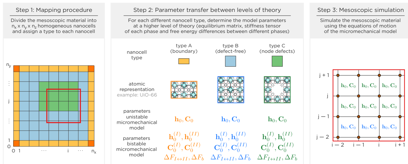
Fig. 2 The three steps in the micromechanical model, illustrated for UiO-66 containing nodal defect regions (green), defect-free regions (blue) and surface regions (orange). Step 3 shows a zoom in of the model on region defined by the red rectangle of step 1.
