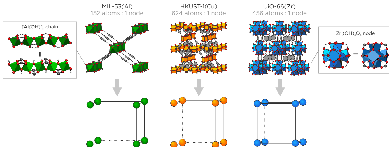
Fig. 3 The micromechanical procedure to map the atomistic model onto the nanocells for three representative MOFs, MIL-53(Al), 54 HKUST-1(Cu), 55 and UiO-66(Zr), 56 with corresponding reduction in the number of degrees of freedom. Insets show the atomistic representations of the inorganic moieties in MIL-53(Al) (left) and UiO-66(Zr) (right). Colour code: zirconium (blue), copper (orange), aluminium (green), oxygen (red), carbon (grey) and hydrogen (white). Hydrogen atoms are omitted from the periodic materials for clarity.
