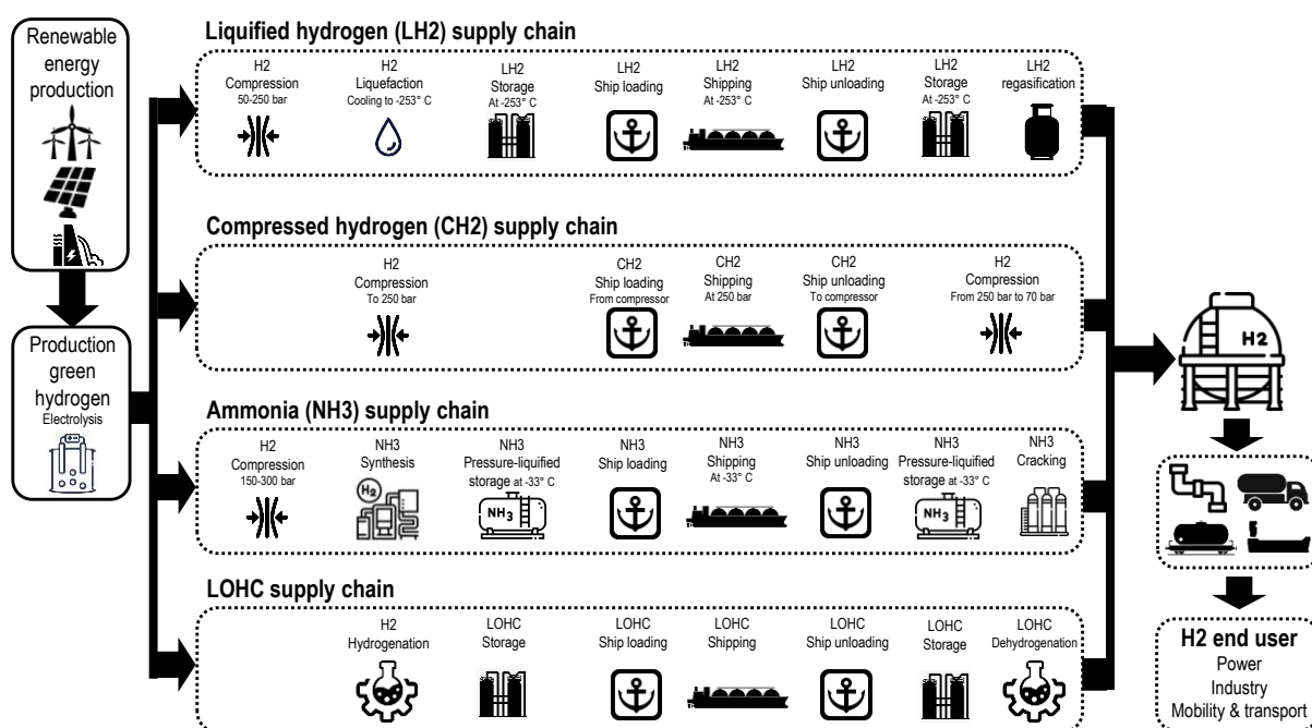
Figure 1. Most considered supply chain solutions for the import of green hydrogen produced overseas
