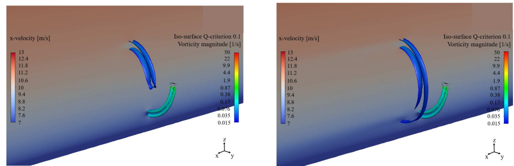
Figure 14. Visualization of the wake after (left) the first loop and (right) the last loop for the crosswind flight with logarithmic inflow. Note that the flow is from right to left. From the contour plot of the x-velocity, the logarithmic profile is clearly visible, but this is disturbed when the aircraft wing passes through this plane due to induced flow. From the flow field after the last loop, it can be seen that there is a velocity deficit in the downstream direction.
