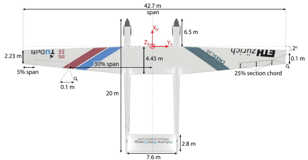
Figure 1. Multi-MW AWE reference system [16].
